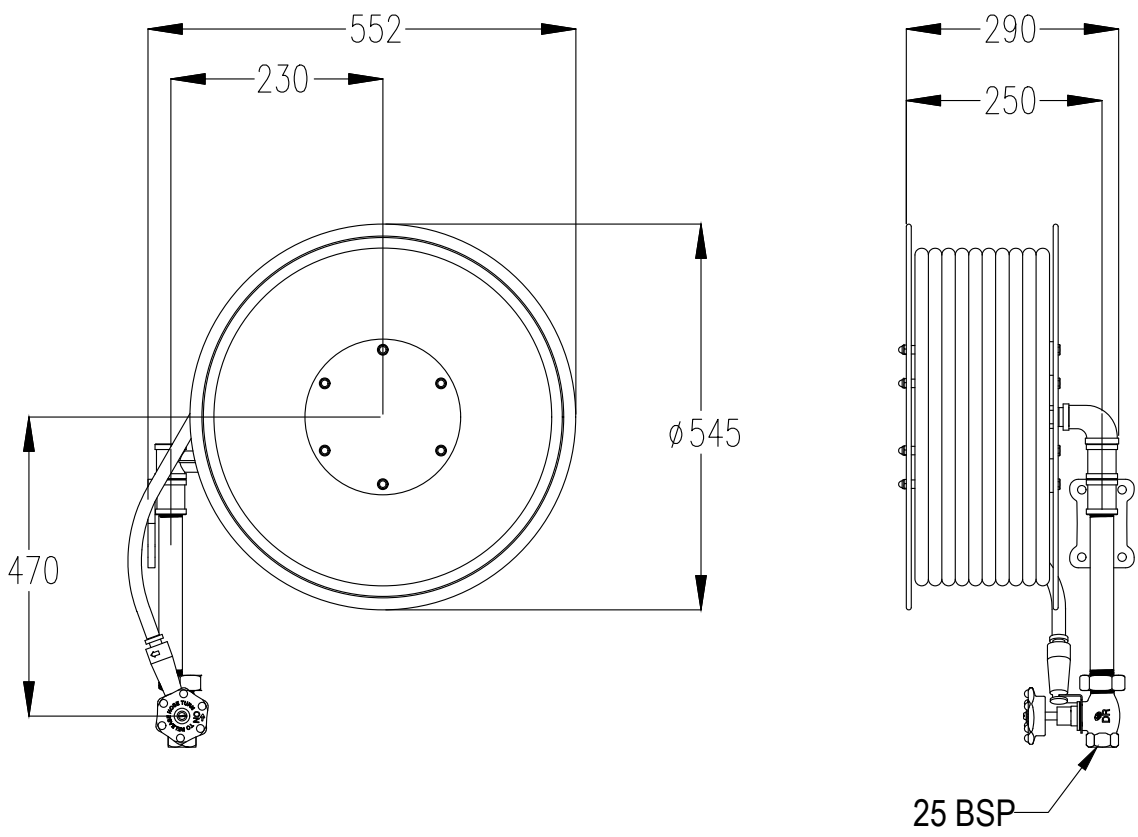
FIRE HOSE REEL DETAIL NOT TO SCALE
