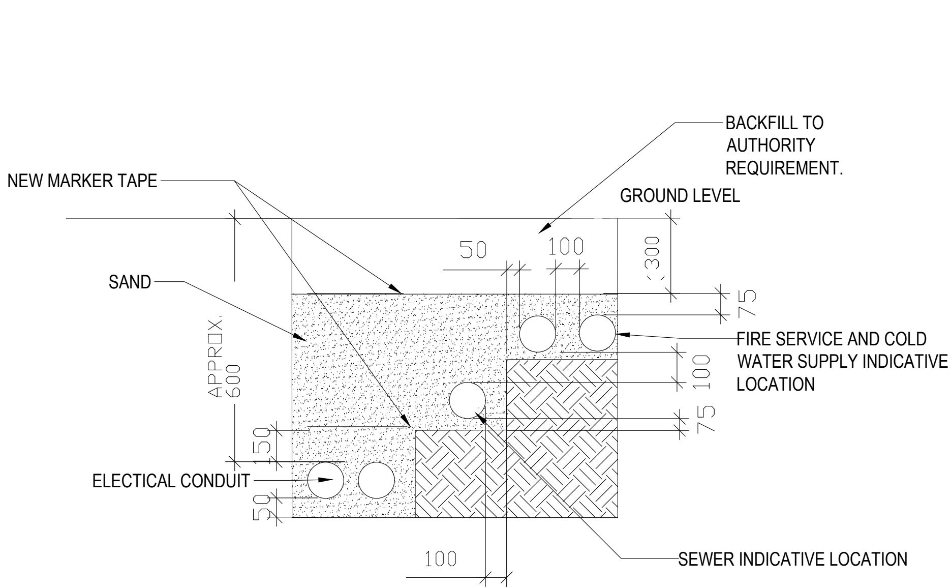
SHARED TRENCH DETAIL NOT TO SCALE
