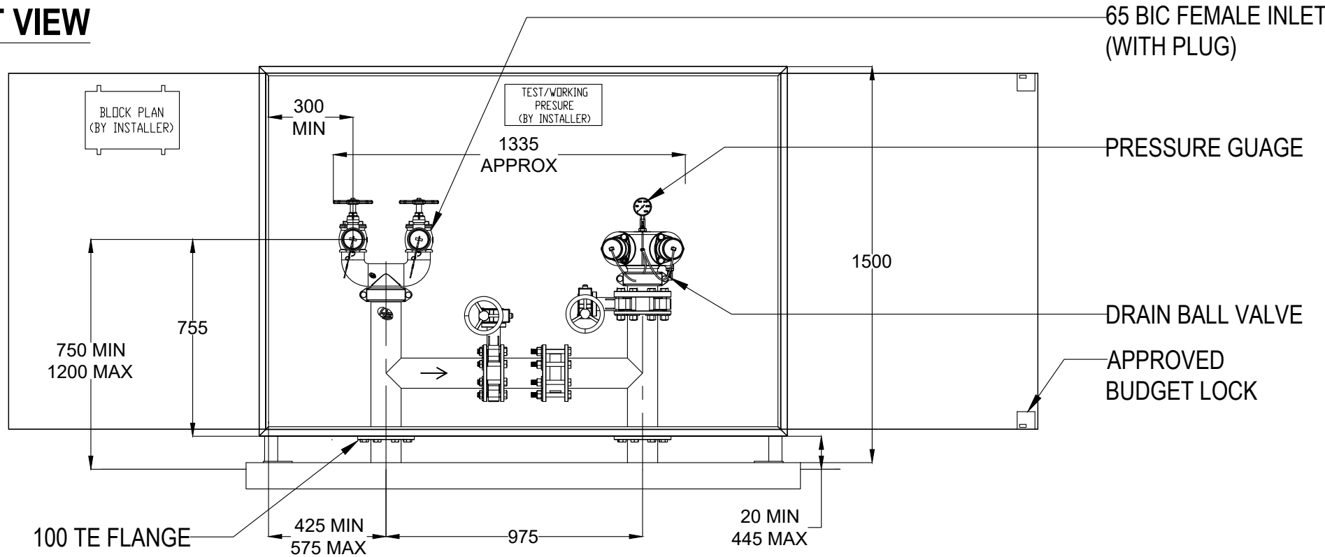
H DESIGN BOOSTER CABINET DETAIL NOT TO SCALE
