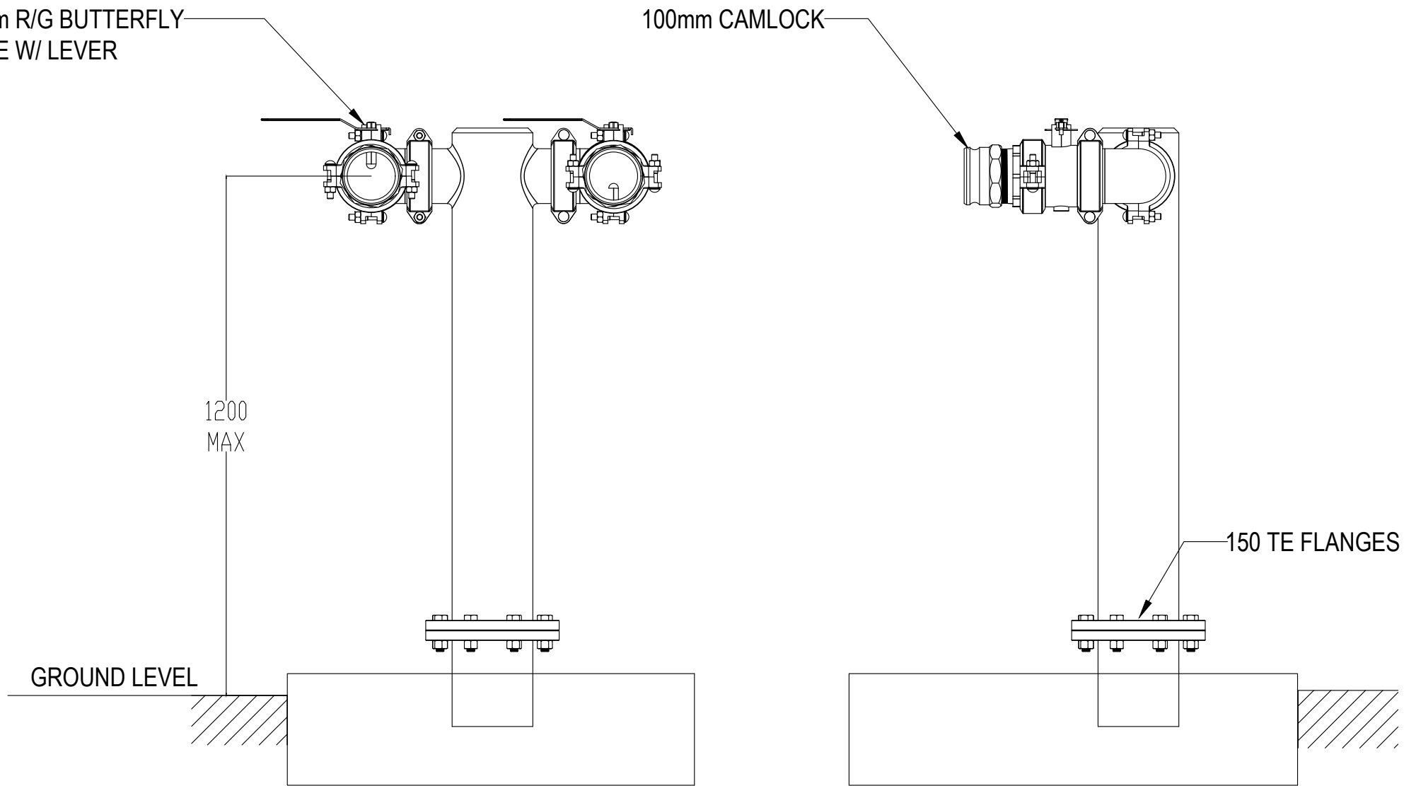
FIRE HYDRANT DETAIL NOT TO SCALE
